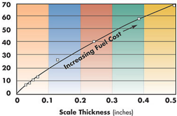
Fuel Cost Increases Due to Boiler Scale
